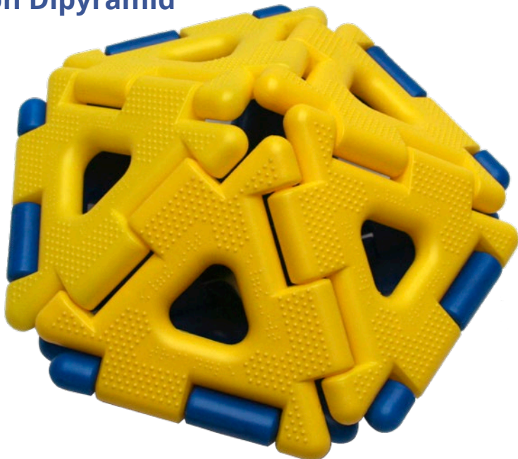
Pentagon Dipyramid
